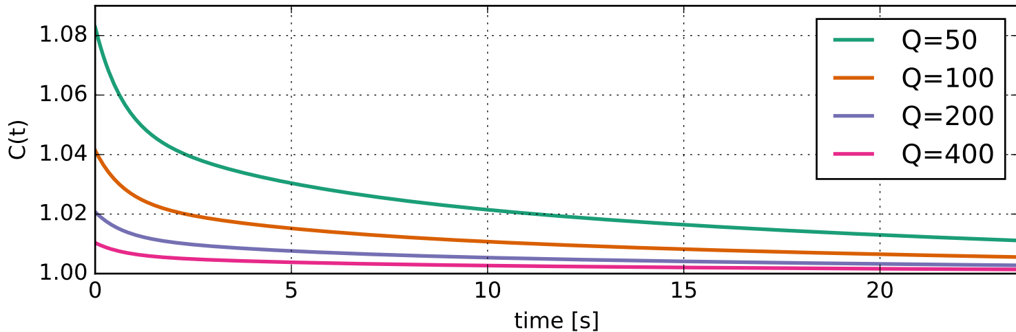
Stress Relaxation Functions
